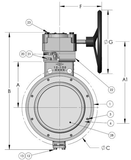
10" 150 WAFER SHOWN
